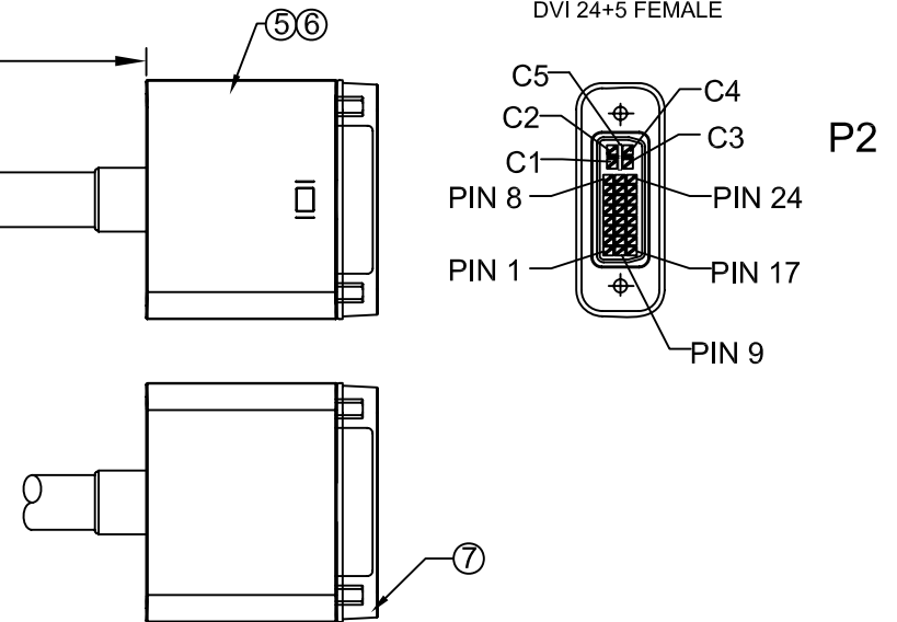
DVI 24+5 FEMALE
